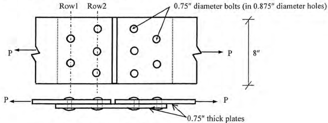
Fig: Bolted joint subjected to force P
