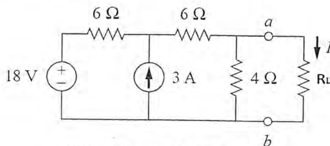
Circuit diagram for question 6(b)
