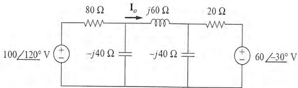
Circuit diagram for question 6(a)
