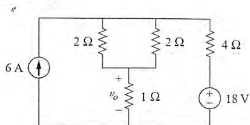
Circuit diagram for question 3(b)
