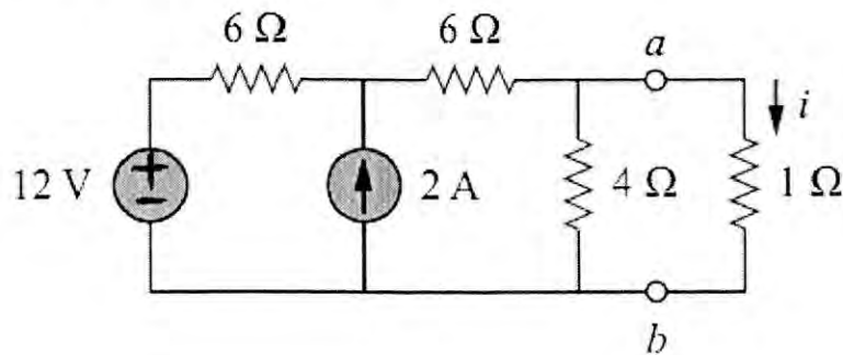
Circuit diagram for question 4(b)
